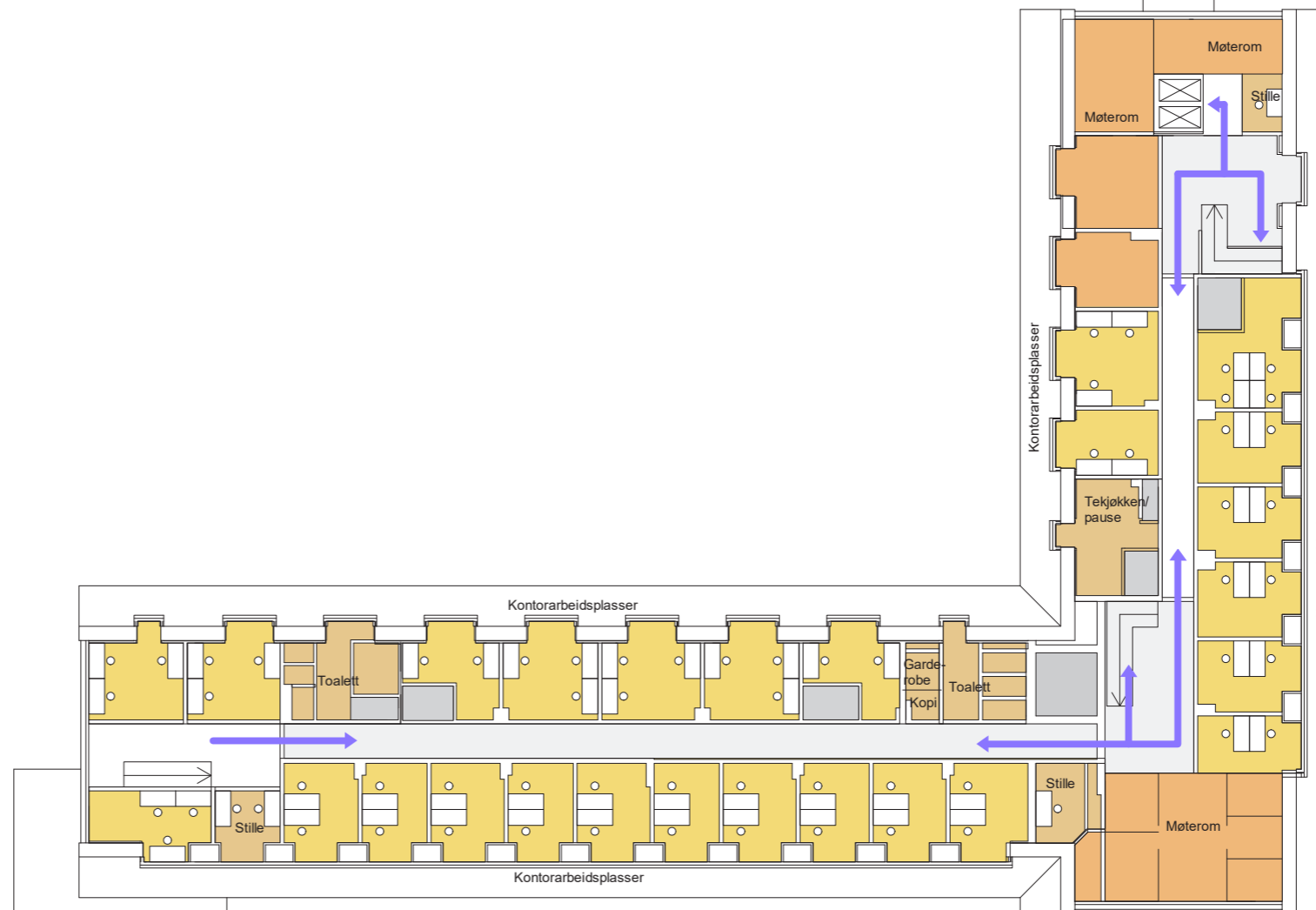
PLAN 11, 12, 13 KONTORER
